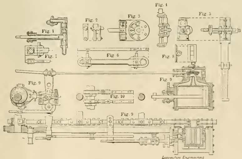
DETAILS OF WINANS' DELAWARE.
